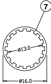
WASHER DETAIL
