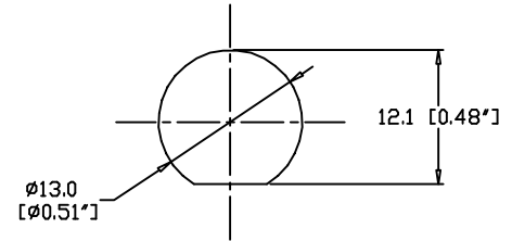
MOUNTING DETAILS
