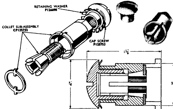
Unsupported collet assembly 418/1/08010 (JS Cat. No. 5355-99-942-8697)
