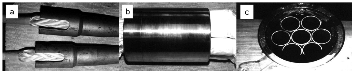
205 206 Fig. 4. Photographs of different termination with rope (a. Parafil socket, b. Viking 7 socket, c. 207 stress relief socket)
