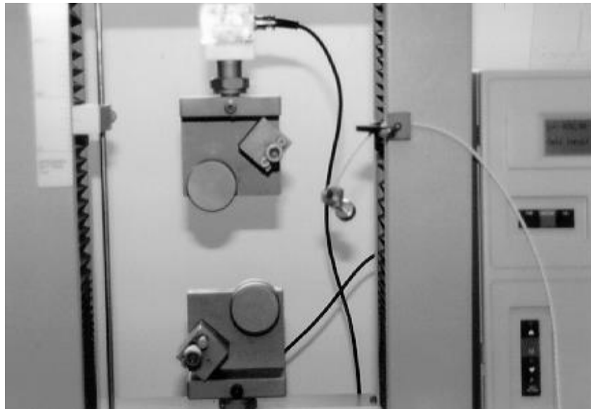
Fig. 2. 5 kN Lloyds Machine used for tensile testing of filaments, yarns and strands.
