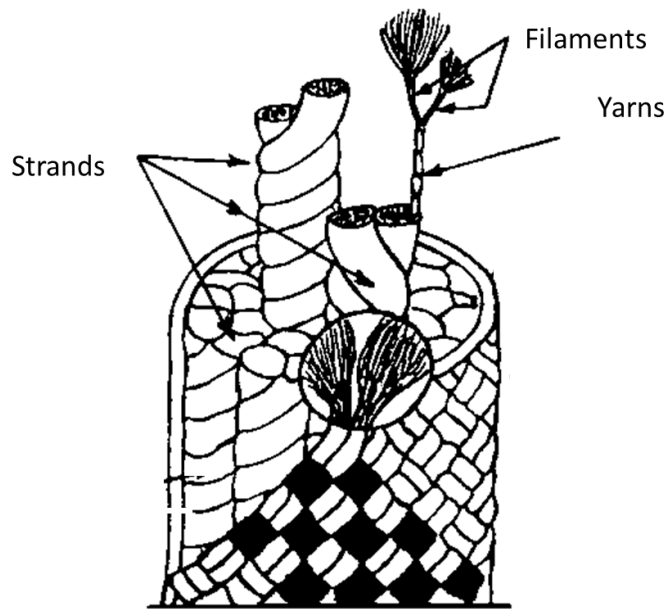
Fig.1. Schematic diagram of rope construction [Natural Disaster Organization, 1996].
