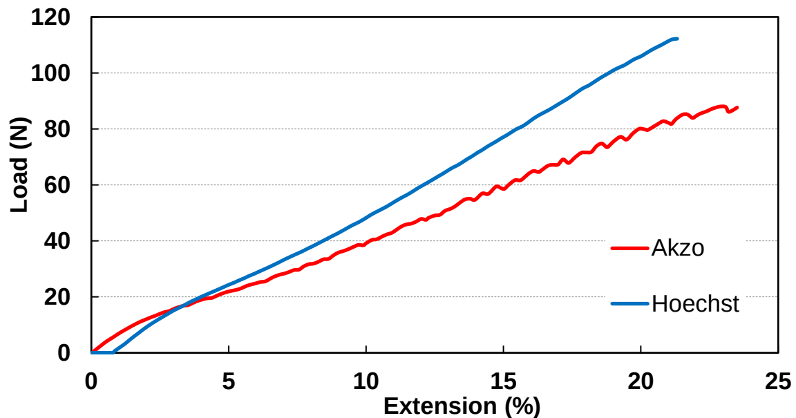
Fig. 7. Typical Load-Extension curve for Akzo and Hoechst filaments.
