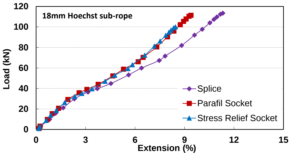
Fig. 9. Load-extension behaviour of 18mm Akzo and Hoechst sub-rope tested with different termination type.
