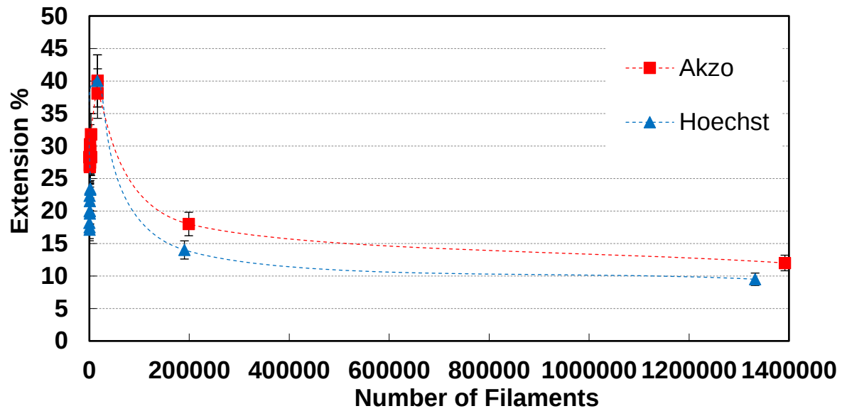
Fig. 11. Extension percentage at break for different number of filaments of Hoechst and Akzo materials.
