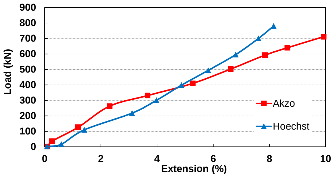
418 419 Fig. 10. Typical load-extension behaviour of 44mm Akzo and Hoechst rope tested with Stress 420 Relief Socket.
