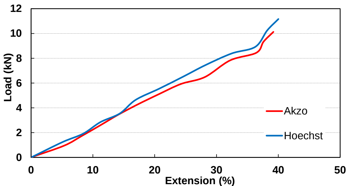
Fig. 8. Typical Load-extension curve for Akzo and Hoechst strands.
