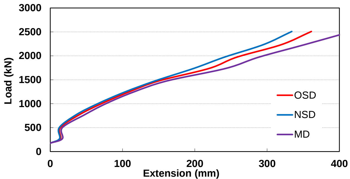
Fig 13. Typical load-extension profile for the 120mm rope samples. (OSD= Offside Displacement transducer; NSD= Nearside Displacement transducer; MD= Machine Displacement).
