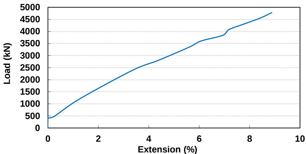
Fig. 14. Typical Load-Extension curve for 120mm rope.
