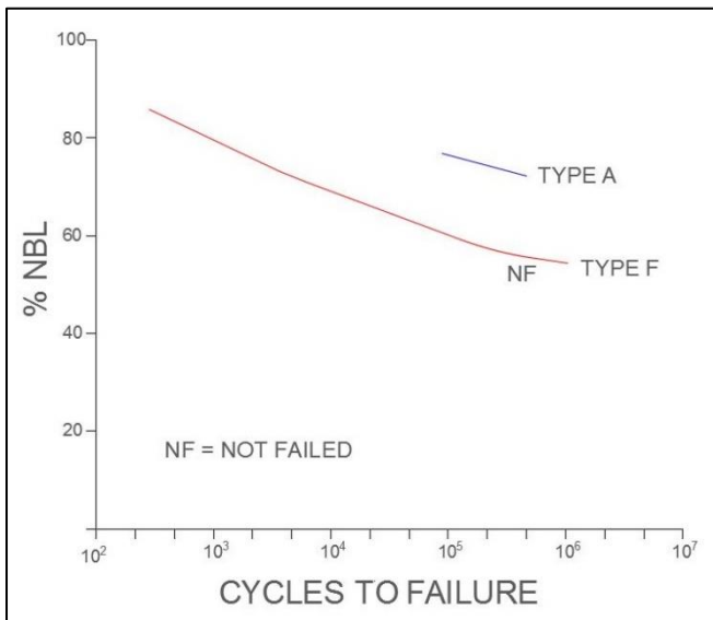
Figure 15 ~ Tension-Tension Fatigue Performance of Parafil® Ropes
