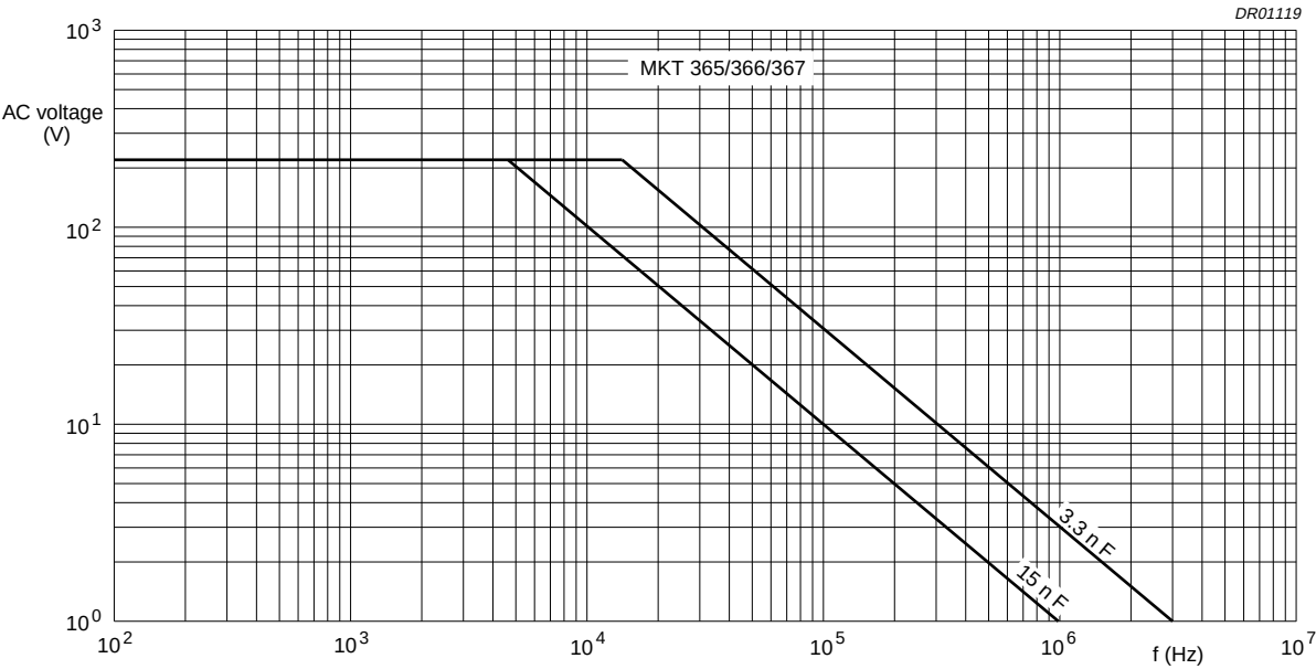
Fig.37 AC voltage (RMS value) as a function of frequency at T_{\text{amb}} \leq 85\text{ }^{\circ}\text{C} , for U_{\text{Rdc}} = 400\text{ V} (2222 365, 366 and 367 styles).
