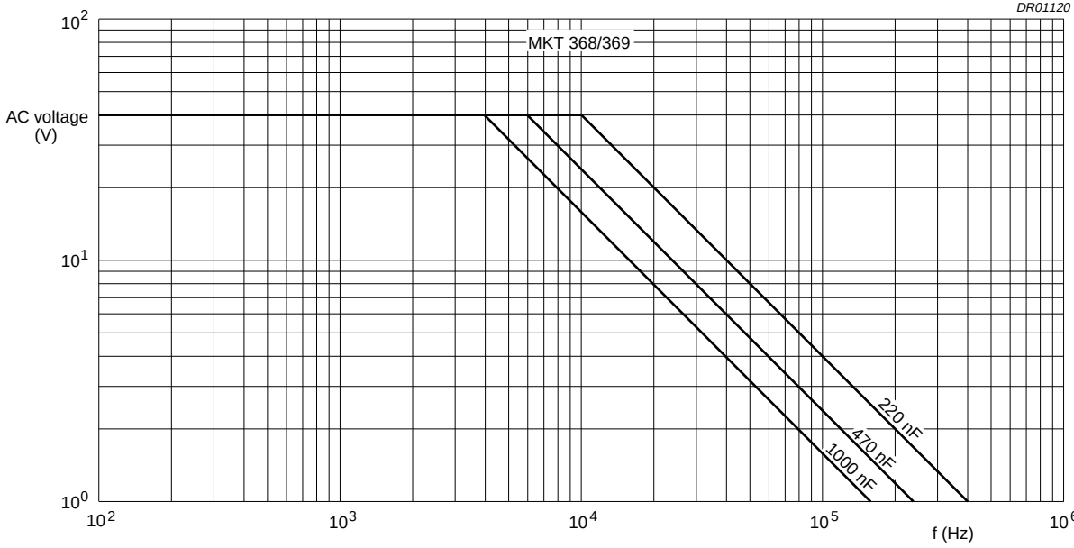
Fig.38 AC voltage (RMS value) as a function of frequency at T_{\text{amb}} \leq 85\text{ }^{\circ}\text{C} , for U_{\text{Rdc}} = 63\text{ V} (2222 368 and 369 styles).
