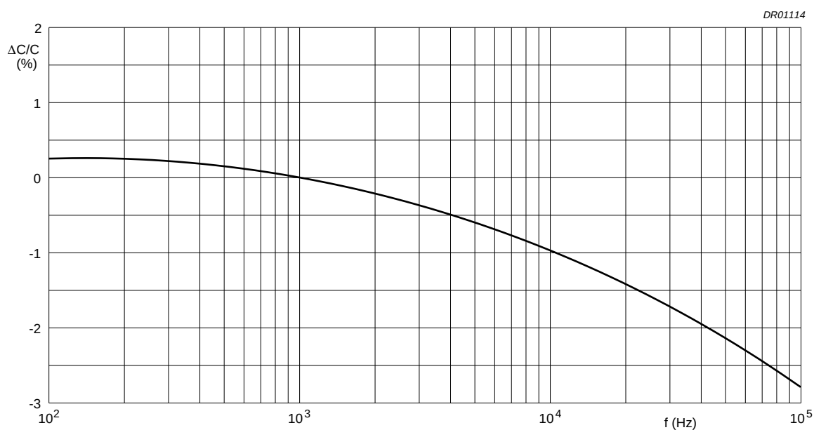
Fig.31 Capacitance as a function of frequency: typical curve.
