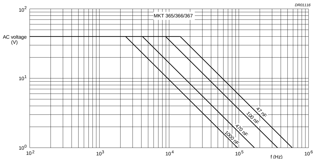
Fig.34 AC voltage (RMS value) as a function of frequency at T_{\text{amb}} \leq 85 °C for U_{\text{Rdc}} = 63 V (2222 365, 366 and 367 styles).
