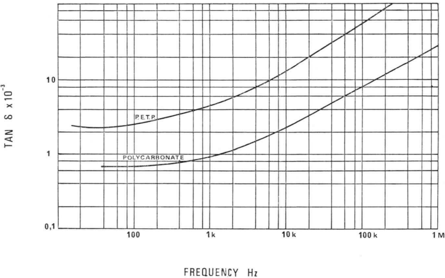
Fig. 8 Variation of Tan \delta with Frequency (measured at 20°C).
