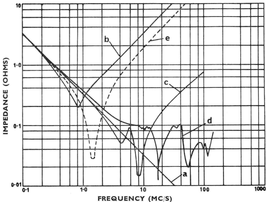
IMPEDANCE-FREQUENCY CHARACTERISTICS OF VARIOUS TYPES OF SUPPRESSORS
