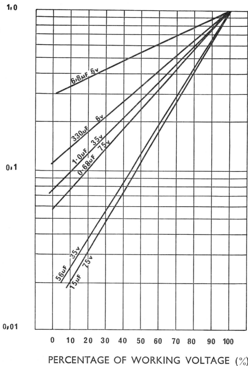
Fig. 10 Variation of leakage current with voltage
