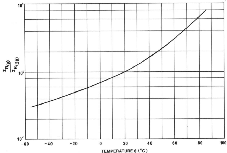
Fig. 7. Variation of Leakage Current with Temperature
