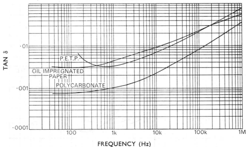
Fig. 6.—Variation of Tan \delta with Frequency (measured at 20°C)
