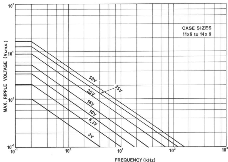
Fig. 10. Variation of Ripple Voltage with Frequency
