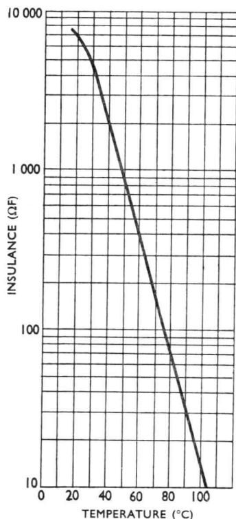
VARIATION OF INSULATION WITH TEMPERATURE
