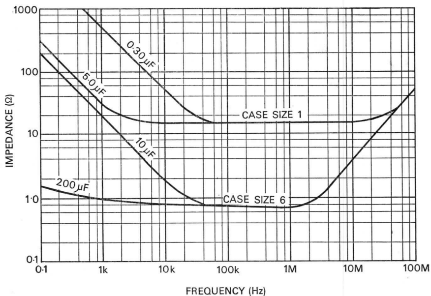
Fig. 4.—Impedance/Frequency Characteristics
