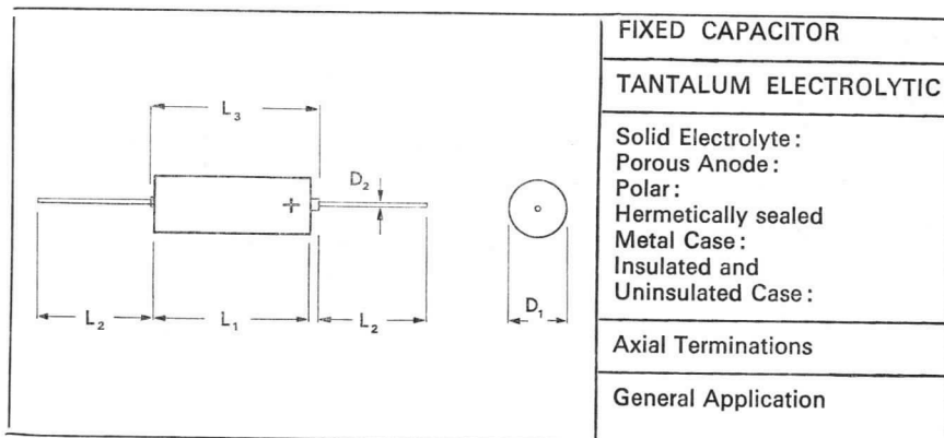
DIMENSIONS uninsulated capacitors
