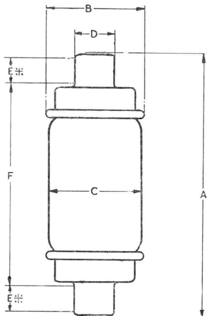
K50/2L and K100/2L Outline
