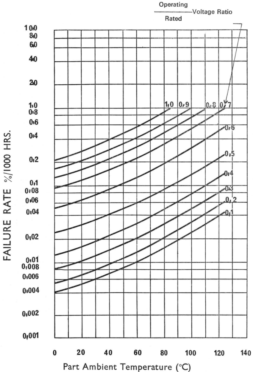
Fig. 11 Effect of temperature and voltage derating on failure rate at 0,1 \Omega/\text{volt} . Compiled from MIL HDBK 217A, Figs. 7.6.34.A
