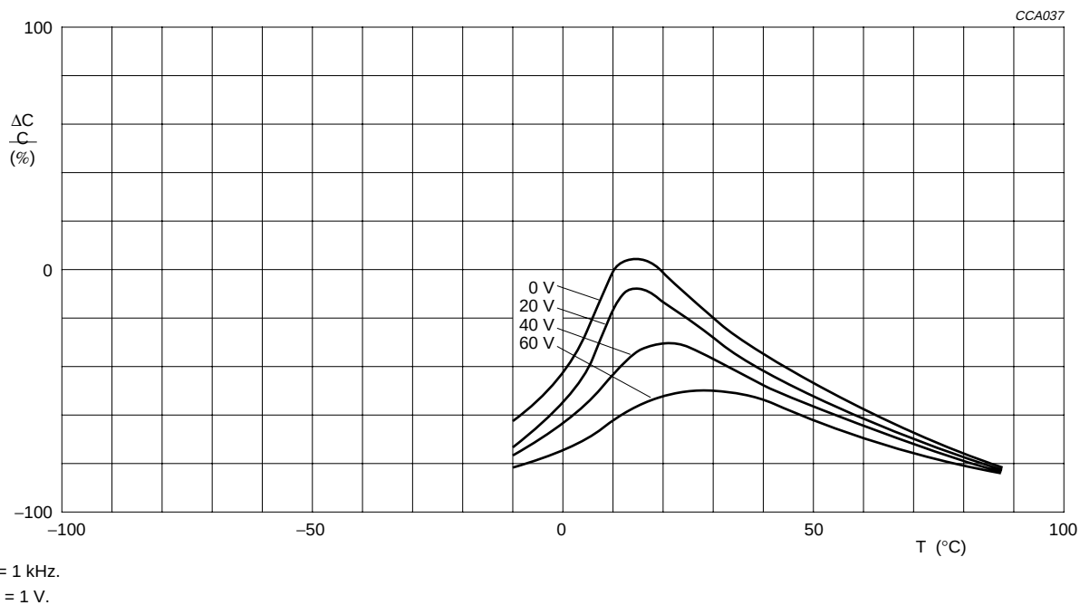
Fig.18 Typical capacitance change with respect to the capacitance value at 0 V and 20 °C as a function of temperature at different DC voltages for capacitance values 2200 to 47000 pF.
