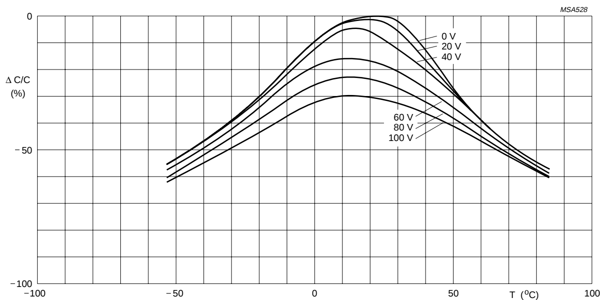
Fig.13 Typical capacitance change with respect to the capacitance value at 0 V and 20 °C as a function of temperature at different DC voltages.
