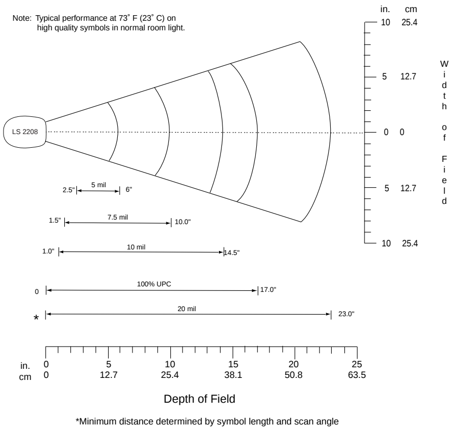
Figure 2-4 Symbol LS2208 Decode Zone
