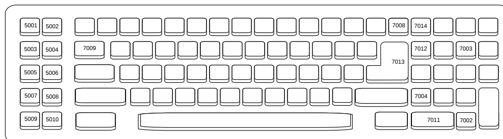
Figure 5-3 IBM PC/AT
