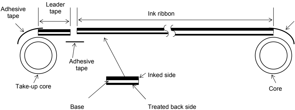
Fig. 3: Connection between Leader Tape and Ribbon
