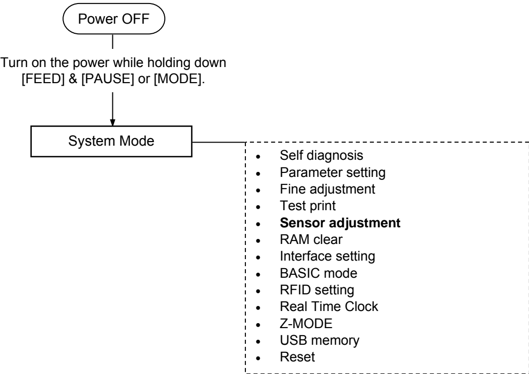
Contents of the Sensor Adjust Menu
