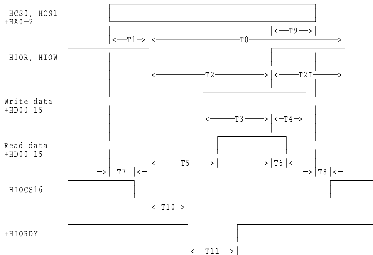
Figure 6-5. PIO cycle timings
