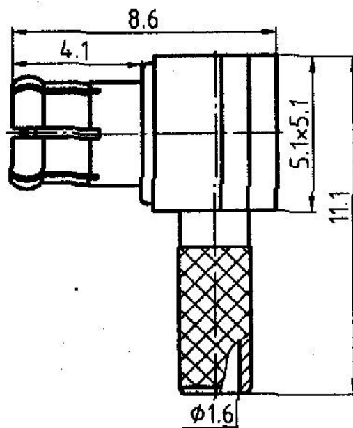
CRIMP FERRULES
