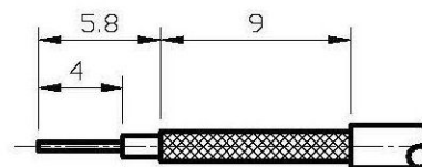
RECOMMENDED STRIP LENGTHS
