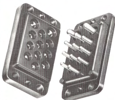
12-pole L655/P Plug L655/S Sockets L655/C3 Cover L655/R3 Retainer
