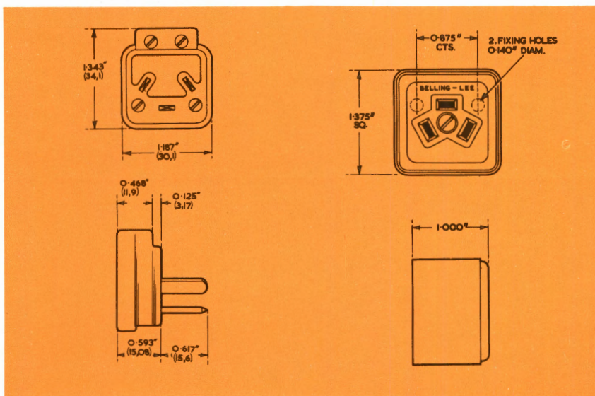
L 374 Free Plug L 303/P Free Plug L 303/F Fixed Socket L 303/S Fixed Socket
