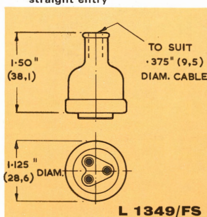
L 1349/FS Free Socket, straight entry
