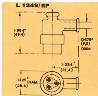
L1349/RP Free Plug, right-angle entry
