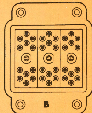
Example B shows three L 1389 Miniature Unitors giving 36 poles in an area of only 1.32 sq. inches.
