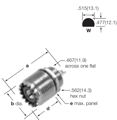
UHF Panel Receptacles 83-1R or 83-1R-RFX 83-798
