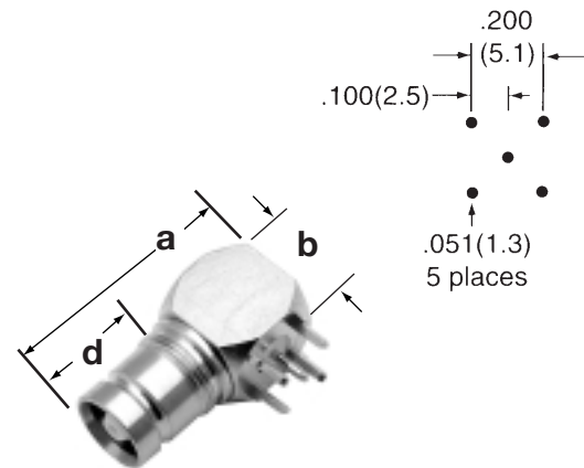
Bulkhead Jacks 156-931-02, 156-931-34, 156-642-RG59
