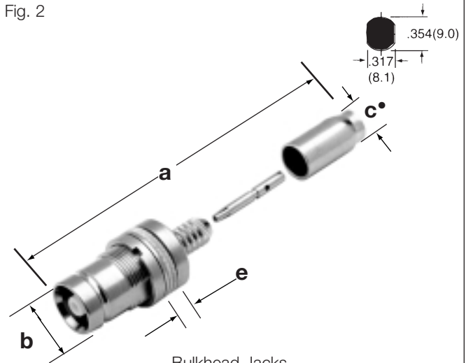
Bulkhead Jacks 156-931-02, 156-931-34, 156-642-RG59
