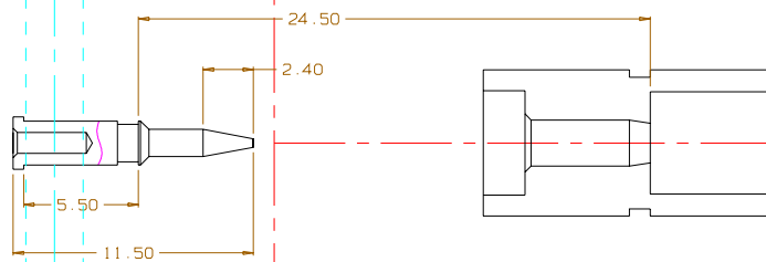
NEW ZL-6001-2 BNC Crimp Only Pin
