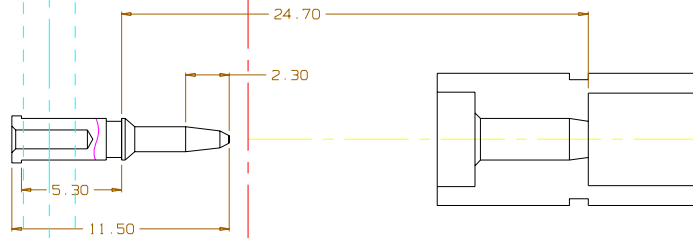
CKT-Updated/Lengthened BNC82 Pin (wrong-changes)
