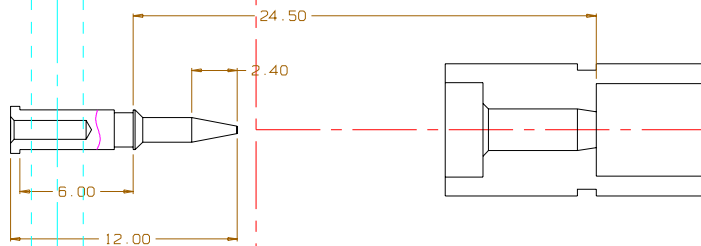
CKT Original BNC Crimp/Solder Pin
