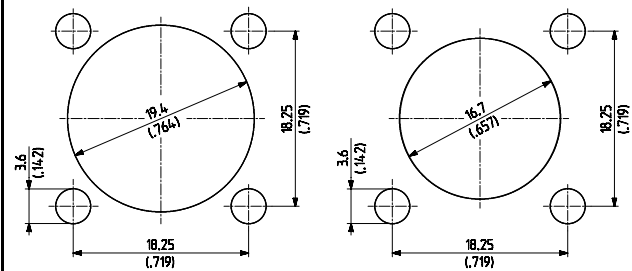
rear panel mounting
