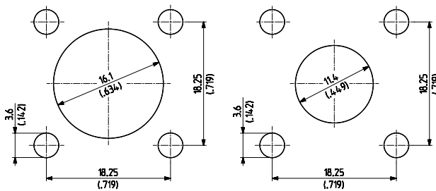
rear panel mounting
