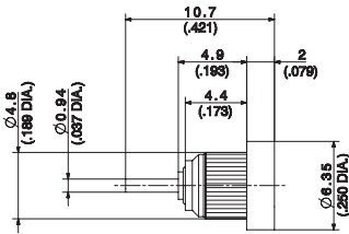
Fig. 2 (press-in)
