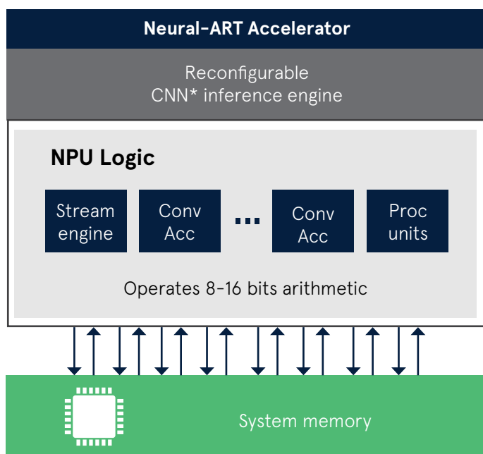
Figure 1: Neural-ART Accelerator architecture
