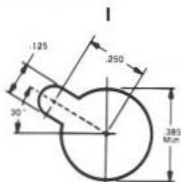
Four-Contact 126-214, 126-214-1001, 126-233, 126-215-1002 only
