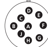
9-96* 9 size 16
