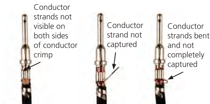
Unacceptable Crimps
