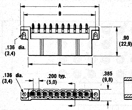
STRAIGHT PIN HEADER
