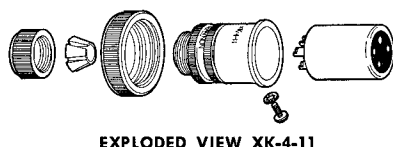
EXPLODED VIEW XK-4-11
