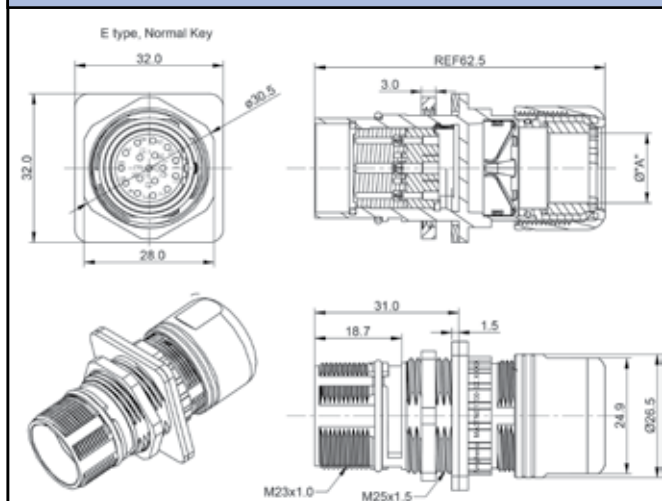
Receptacle, Bulkhead, Threaded, 11-15mm Cord Grip
