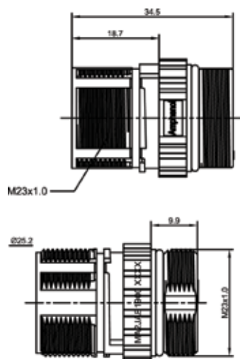
Receptacle extension, straight, Checkmate™
