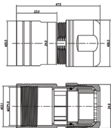
Cord Grips
