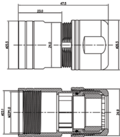
Cord Grips
