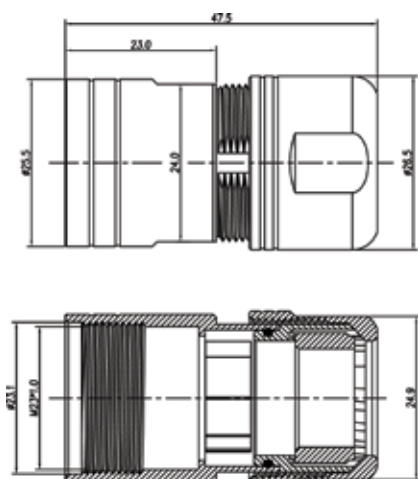
Cord Grips
