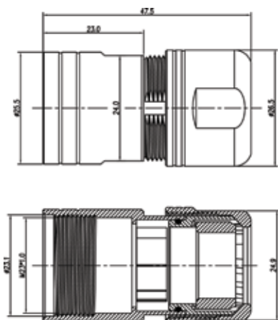
Cord Grips
