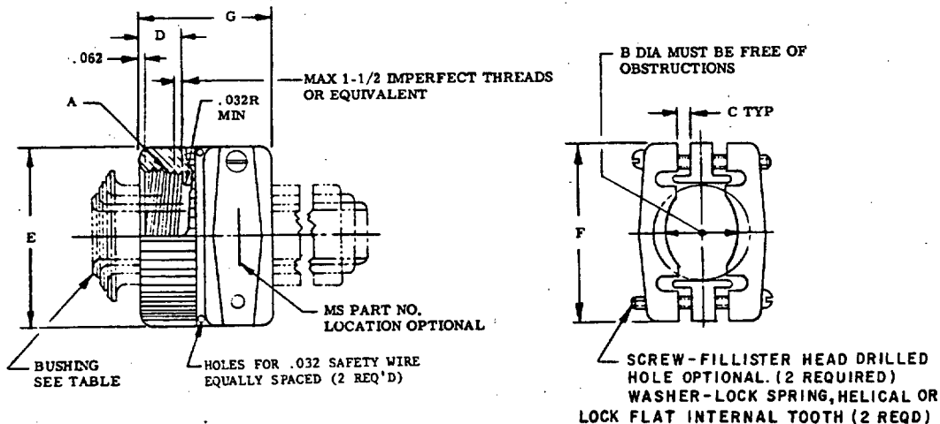
TYPE A - CABLE CLAMP, STRAIN RELIEF
