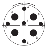
14-9 5 # 20, 4 # 12, I
