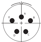
14-5 5 # 16, II
