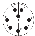
12-8 8 # 20, I
