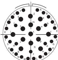
22-41 14 # 16, 27 # 20, I
