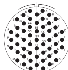
22-55 55 # 20, I
