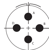
14-4 4 # 12, I
