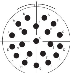
22-21 21 # 16, II
