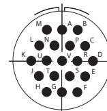
14-19 19 # 20, I
