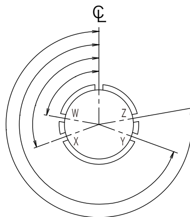
Front face of Pin Insert or Rear face of socket insert
