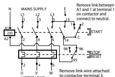
3 Phase 4 Wire Supply – 56MS230
