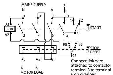
Single Phase & Neutral Supply – 56MS230
