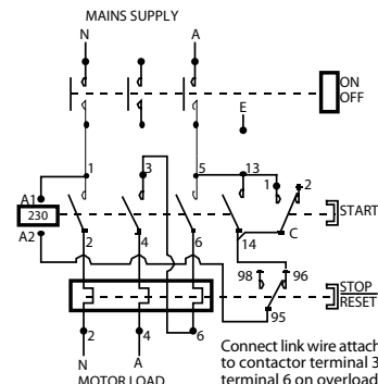
Single Phase & Neutral Supply – 56MS230SW
