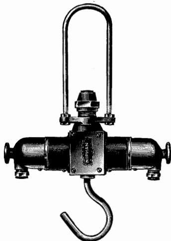
2-WAY HANGING TEE WITH ANGLE PLUGS
