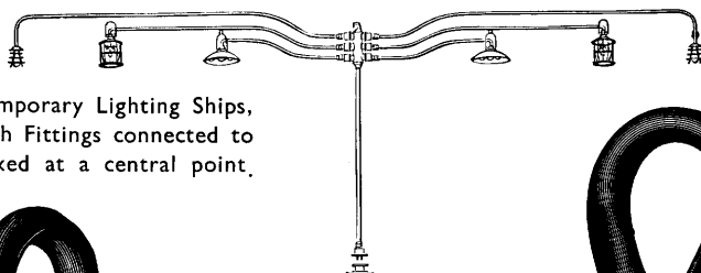
Socket Feed
