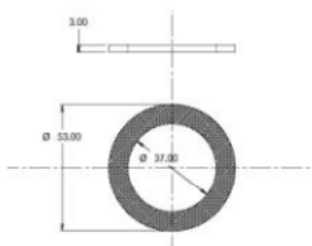
62NIPH-51mm-Gasket_Dwg...
