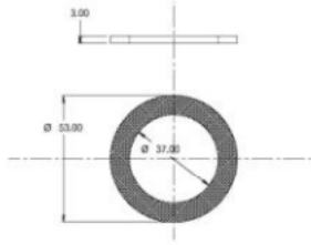
21NIPH-CAP-GASKET-NE3...
