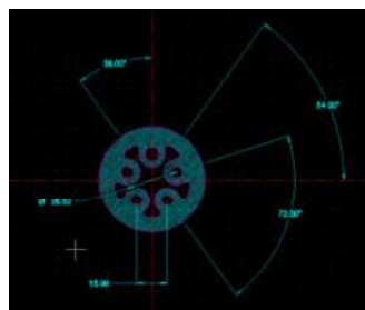
11NIPH-5P-60A-500V-N840...
