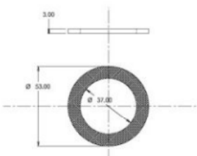
62NIPH-51mm-Gasket_Dwg...
