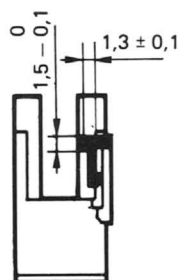
double depth key – black 8613-4102 – grey 8613-4106
