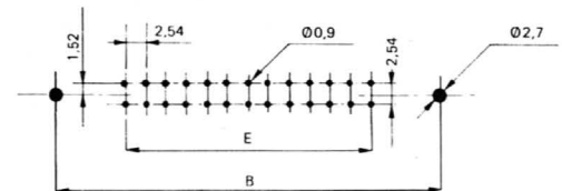
straight spill termination
