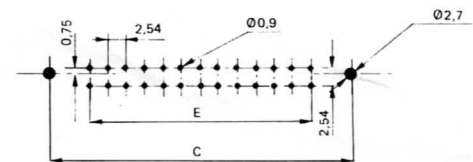
angled spill termination
