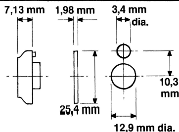
Panel cut-out
