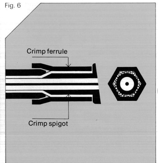
Fig. 6 Crimping outer conductor
