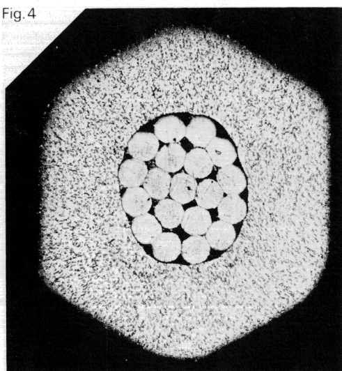
Fig. 4 Crimping in accordance with MIL-C-39012, Category D, Pin 16-10 Pull-out force: 7 kp
