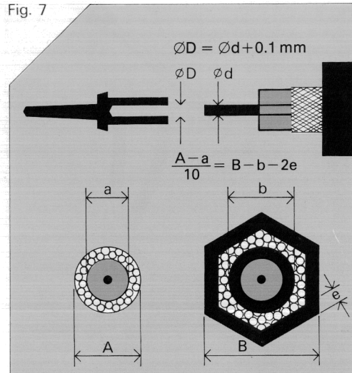
Basic rules for dimensioning crimp components
