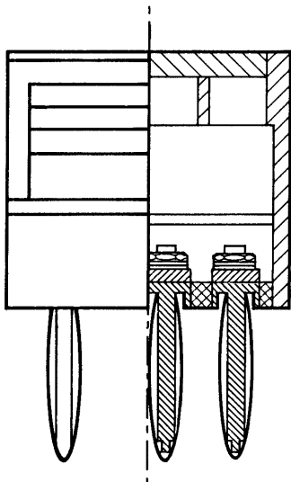
6-pole audio link non-monitoring A-C42334-A9-A8
