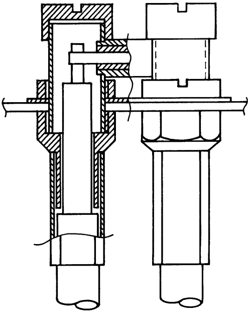
Solid solder – panel mounted A-C42334-A26-A1
