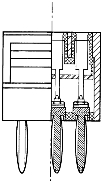
6-pole audio link monitoring A-C42334-A9-A11
