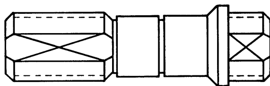
BPO-10 male to SP female A-C42334-A85-A74
