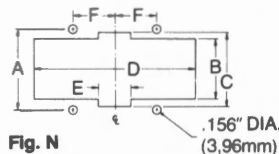
Panel mounting dimensions (suggested)
