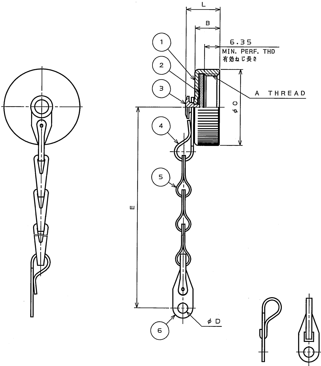
OPTIONAL FORMS FOR PART ④AND⑤ 部品④⑤別形状
