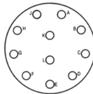
21-11 11 Size 12 Contacts Service Rating I
