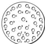
19-30 1 Size 16 Contact 29 Size 20 Contacts Service Rating I
