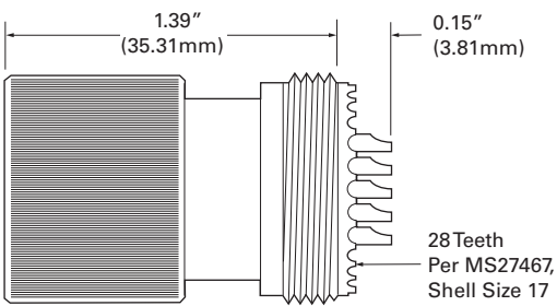
27-Contact Plug
