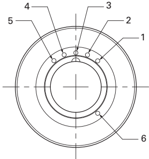
Ground pin locations for panel-mount receptacles
