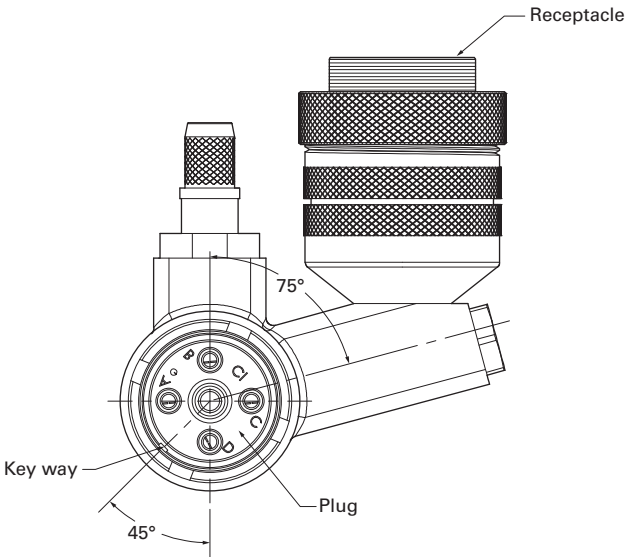
MPAUP/3-4A-2BL175 – The receptacle is oriented to the right with the plug facing forward.
