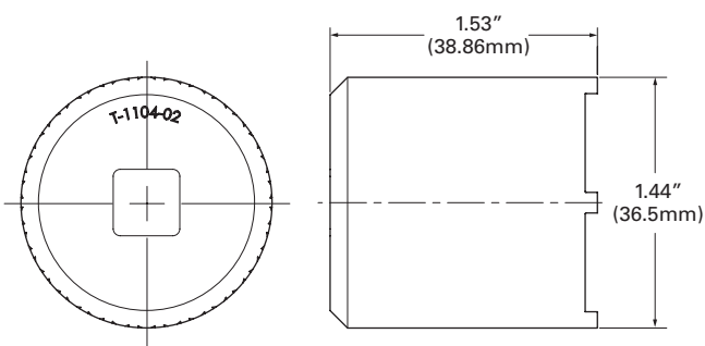
MW20 connectors utilize the T -1104-02 spanner wrench.
