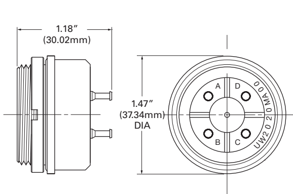
UW2020MA00 receptacle
