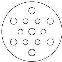
76 insert 7 contacts 20AWG 6 contacts 22AWG
