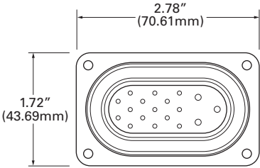
18 Pin Configurations
