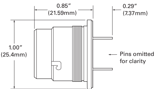
27-Contact Receptacle
