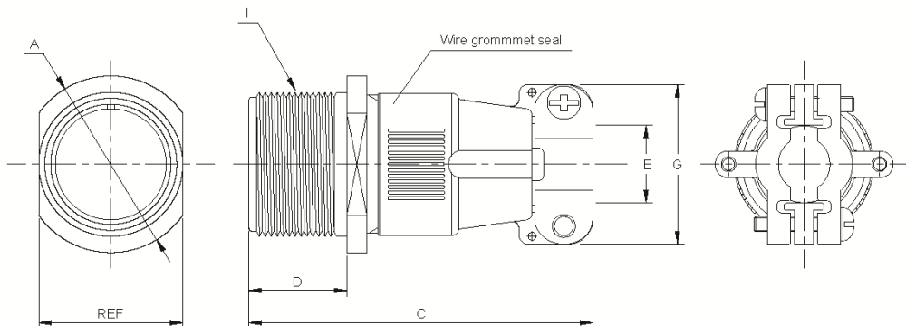
Cable connecting Receptacle
