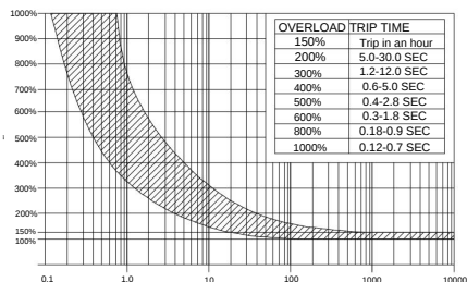
Trip Time Curves
