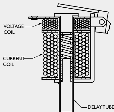
Fig. 28 Dual coil circuit breaker.
