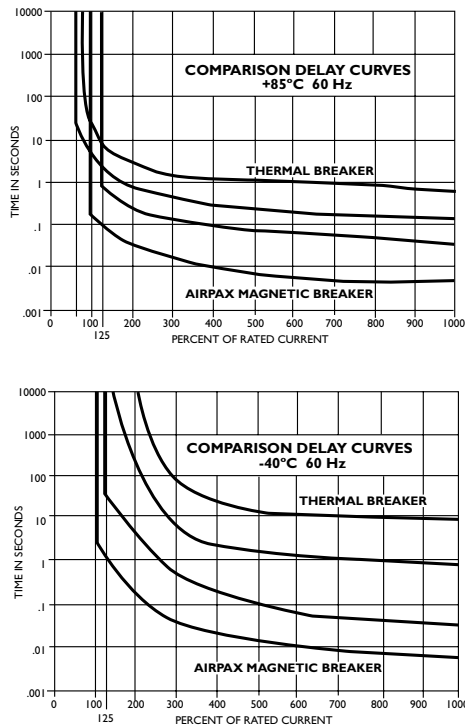
Fig. 8 Magnetic versus thermal breaker characteristics at high and low temperatures.
