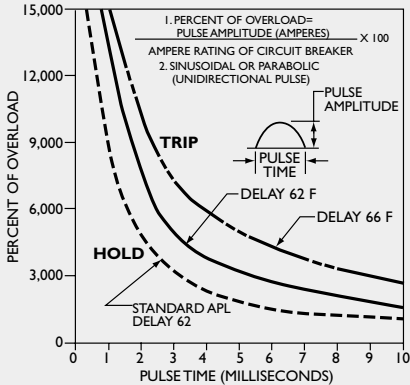
Fig. 18 Percent of overload versus pulse time of an Airpax magnetic breaker.
