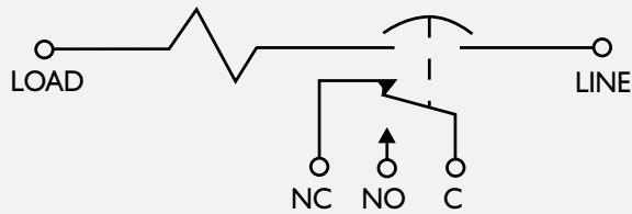
Auxiliary Switch
