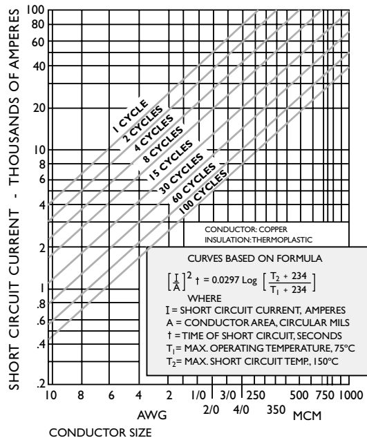
Fig. 13 Short circuit currents for insulated cables.
