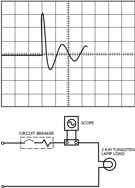
Fig 14 Transient current from a tungsten lamp load.
