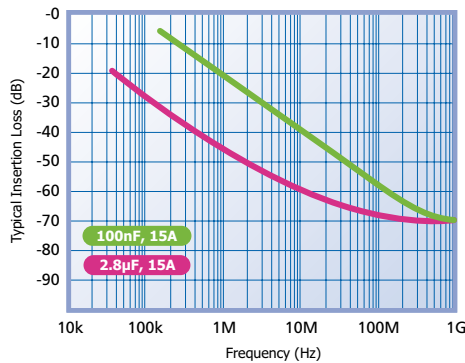
Typical performance in a 50Ω system
