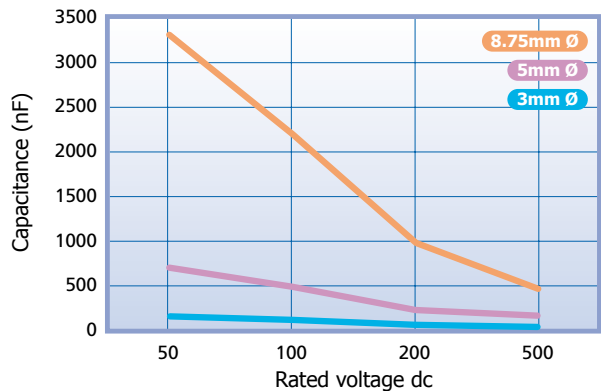
Typical capacitance vs disc size vs voltage Based on typical hole diameter of 0.8mm, and X7R dielectric.
