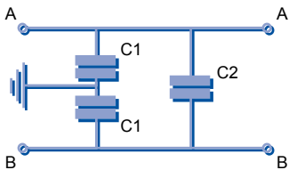
Circuit configuration
