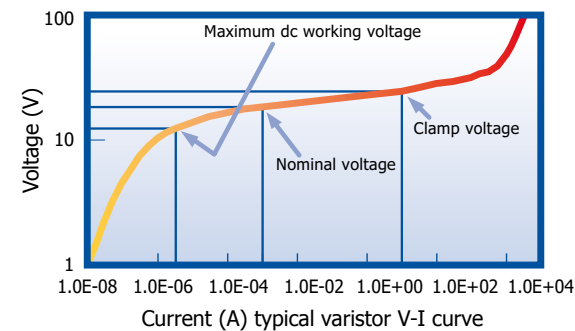
Varistor V-I characteristics
