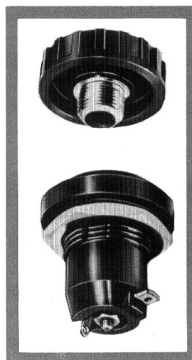
L675 Fuseholder, panel, sealed Qualification approved
