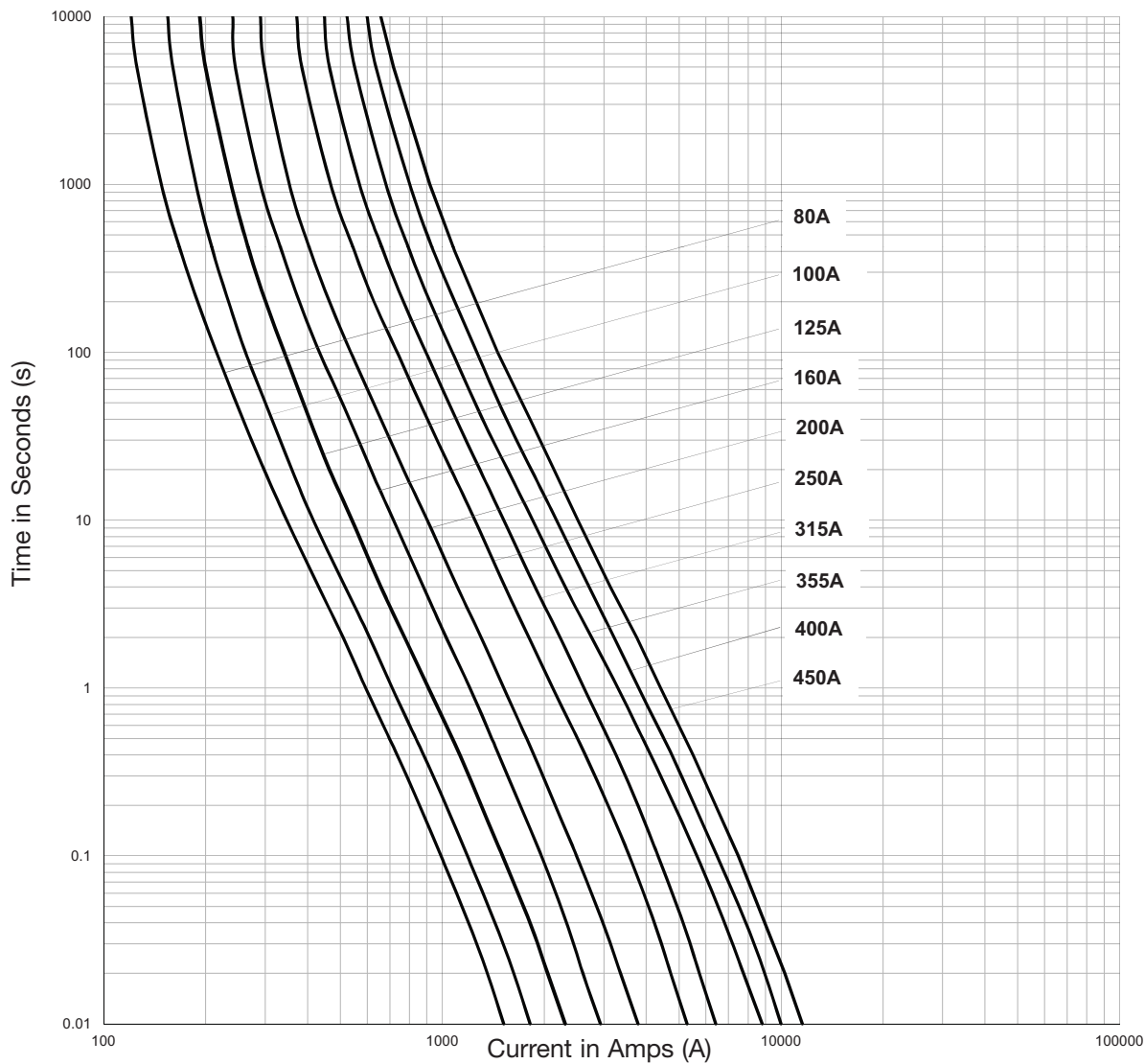
Time-Current Characteristics TC, TF, TKF, TKM, TMF, TM and TTM
