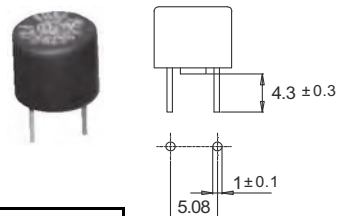
Dimensions [mm]
