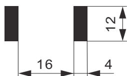
Solder Pad
