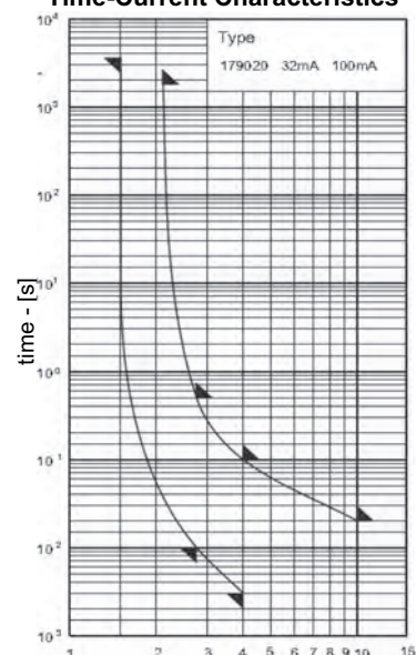
Time-Current Characteristics
