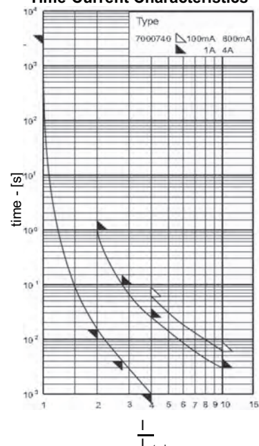
Time-Current Characteristics
