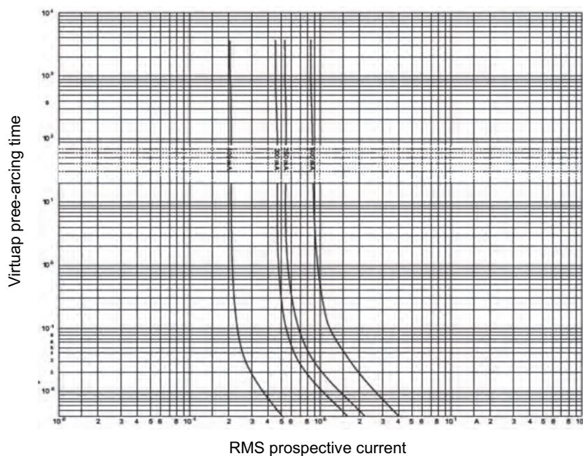
Time-Current Characteristics
