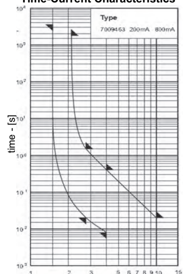
Time-Current Characteristics
