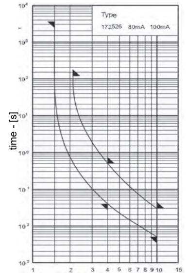
Time-Current Characteristics
