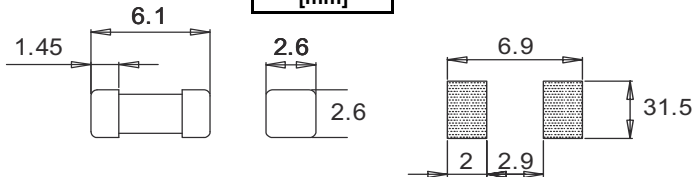
Dimensions [mm]
