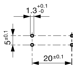
Drill Pattern
