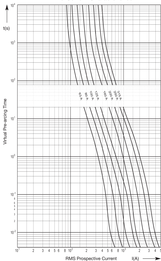
Time-Current Characteristics
