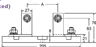
Diagram 2 (1250A Rated)
