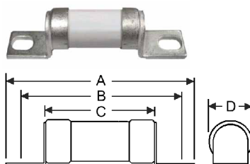
OFFSET TAG Dimensions in MM
