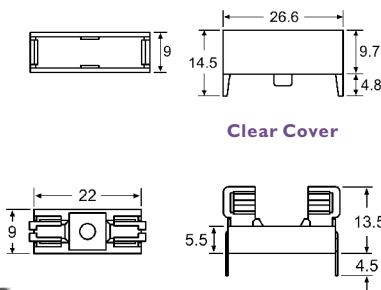
PCB Mount Base
