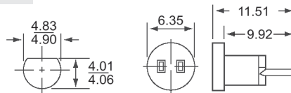
Recommended Mounting Pattern
