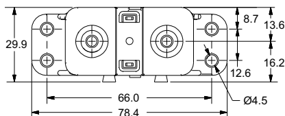
Ganged Fuse Block
