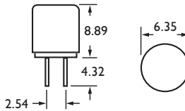
Plastic Cap (273) Short Lead
