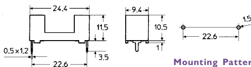
Mounting Pattern
