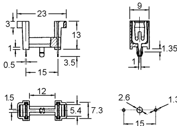
Mounting Pattern
