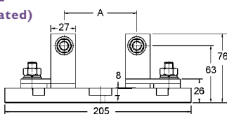
Diagram 2 (1250A Rated)
