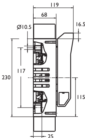
Battery Fuse I-BFxxx
