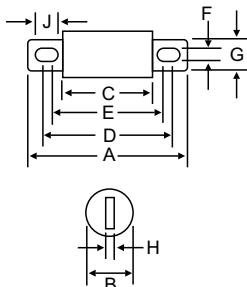
Diagram 1 (5A - 800A)
