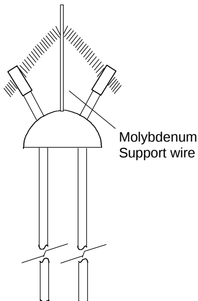
C-2V filament shape (single support)
