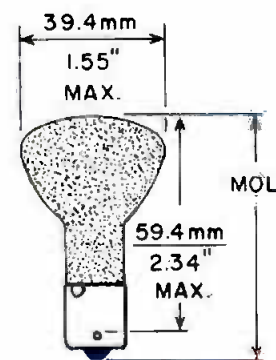
(1/2 size) Fig. 23 R-12
